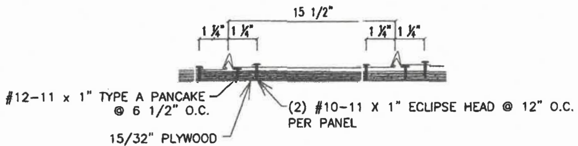
TYPE 2 FASTENER PATTERN (SEE LOAD TABLE)
