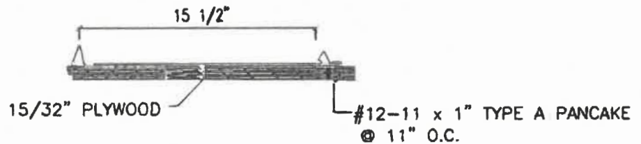
TYPE 2 FASTENER PATTERN (SEE LOAD TABLE)
